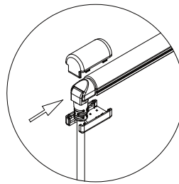
90° (Bottom) Power Cable (NFTB-BS30) Installation
