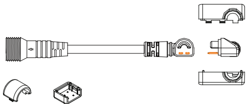
NFSB-ES30 - 1 ft 90° (Side) Power Cable (strip to screw connector)
