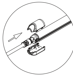
Straight Power Cable (NFTB-TS30) Installation
