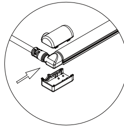
90° (Side) Power Cable (NFTB-ES30) Installation
