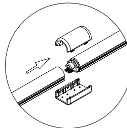
Butt Connector Installation
