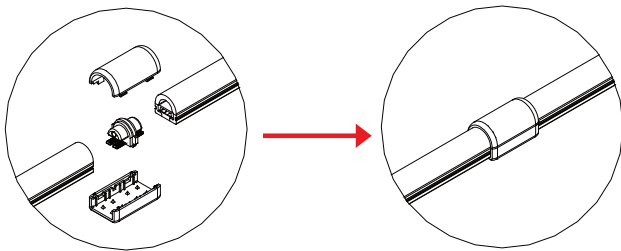
NFTB-CONN - Butt Connector
